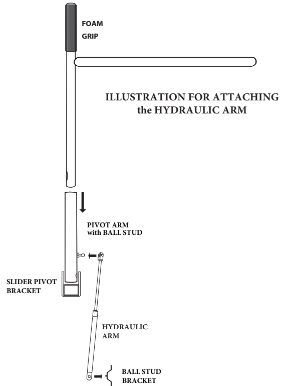
FRONT VIEW - CENTRE POLE ASSEMBLY
